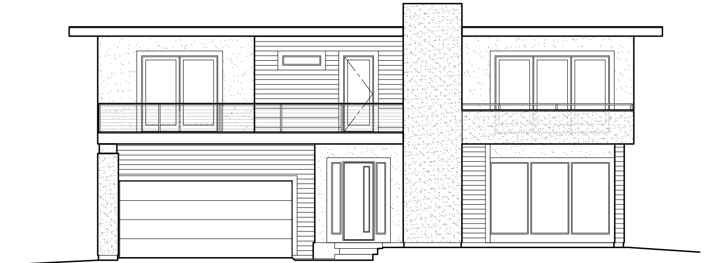
FRONT ELEVATION
